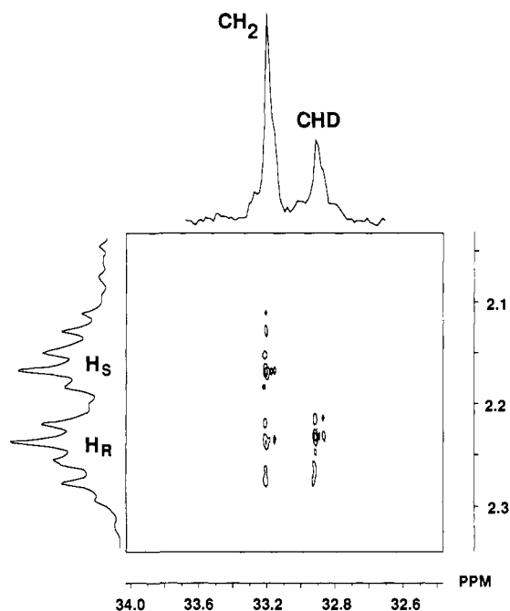
Figure 6. ^2\text{H} -decoupled ^1\text{H} , ^{13}\text{C} shift correlation NMR spectrum of the C-2 methylene group of 10 obtained by degradation of dehydrocurvularin ( 1 ) derived from sodium [2\text{-}^{13}\text{C}, 2\text{H}_3]\text{acetate} . The ^2\text{H} , ^1\text{H} -decoupled ^{13}\text{C} NMR spectrum and ^1\text{H} NMR spectrum are shown on the horizontal and vertical axes, respectively. Spectra were obtained on ca. 0.05 M solutions of 10 in \text{C}_6\text{D}_6 . See ref 33.
