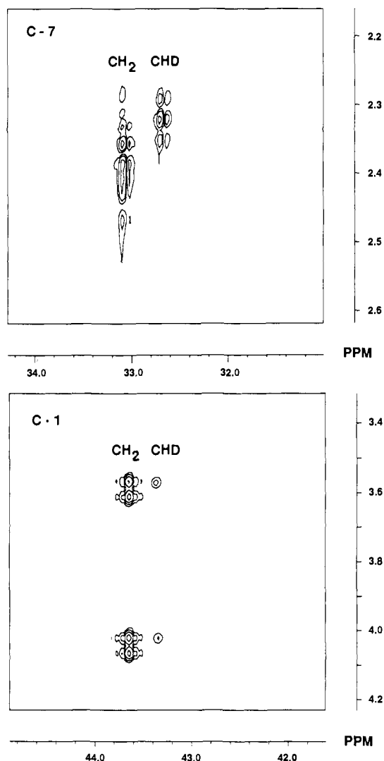
Figure 4. 2 H-decoupled 1 H, 13 C shift correlation NMR spectra of dehydrocurvularin ( 1 ) derived from sodium [2- 13 C, 2 H 3 ]acetate. Upfield CHD correlations show that C-7 is stereospecifically labeled but C-1 is not. Spectra were obtained on ca. 0.15 M solutions of 1 in [ 2 H 6 ]acetone on a Bruker WH400 instrument. See ref 33.
