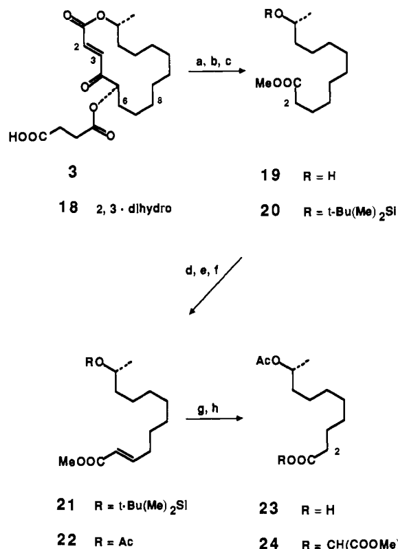
Figure 8. Degradation of A26771B (3): (a) \text{H}_2 , Rh/C; (b) NaOH, \text{O}_2 then HCl, \text{CH}_2\text{N}_2 ; (c) t -Bu(Me) 2 SiCl, imidazole; (d) LDA, PhSeBr; (e) \text{H}_2\text{O}_2 ; (f) \text{Ac}_2\text{O} , FeCl 2 ; (g) NaIO 4 , RuCl 3 ·3H 2 O; (h) methyl ( S )-(+)-mandelate, DCC, DMAP.
