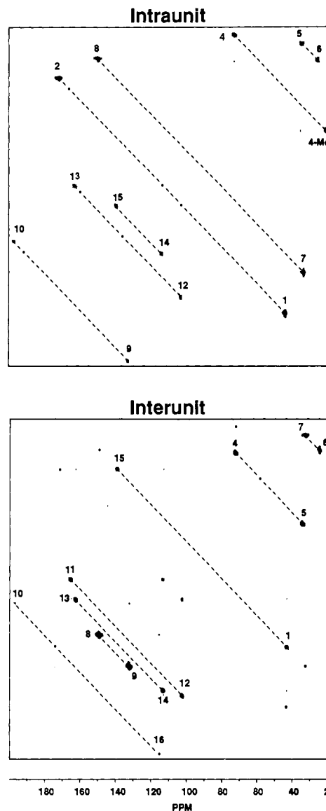
Figure 2. Symmetrized 2D INADEQUATE NMR spectra of dehydrocurvularin ( 1 ) enriched by incorporation of sodium [\text{1,2-}^{13}\text{C}_2]\text{acetate} (upper spectrum) and a 1:1 mixture of sodium [\text{1-}^{13}\text{C}] - and [\text{2-}^{13}\text{C}] -acetates (lower spectrum). Some intraunit coupled carbons can also be seen in the interunit spectrum. The C-11 to C-16 intraunit interaction is present but is not visible at the level shown.
